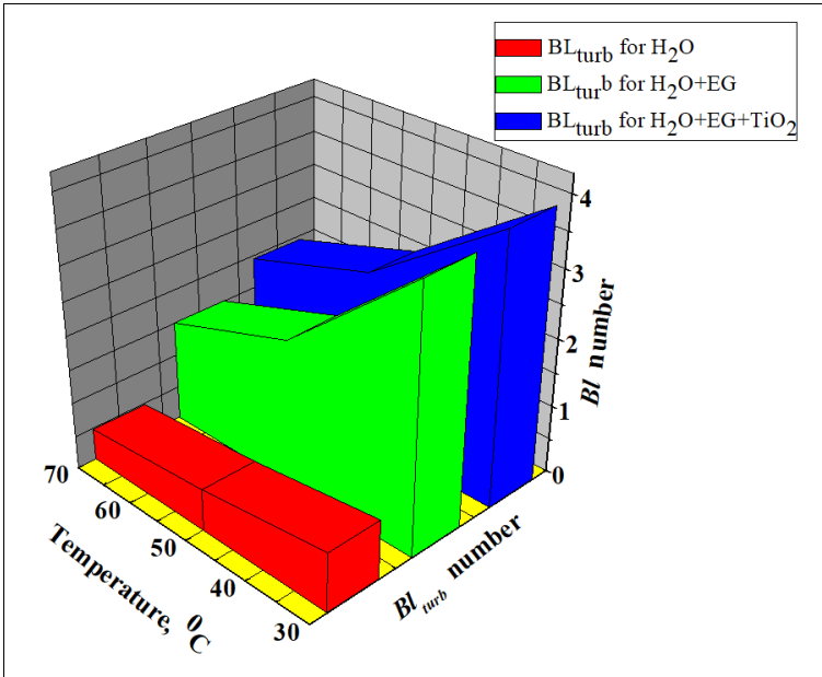
Fig. 4. Influence of the molecular Bl number on the turbulent Bl_{turb} number depending on temperature for various mixes of nanofluidic heat transfer fluids
