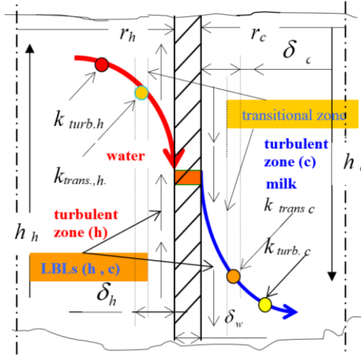
Figure 3. The scheme for transferring the heat through the metal wall from hot water (h) to cold milk (c)
