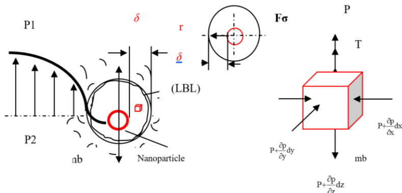
Fig. 2. Scheme of LBL formation around a mobile nanoparticle in a liquid coolant with a T – regime
